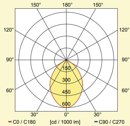
Illustration 94: Downlight
