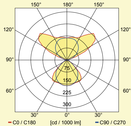
Illustration 97: Luminaire suspendu
