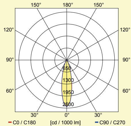
Illustration 95: Spot
