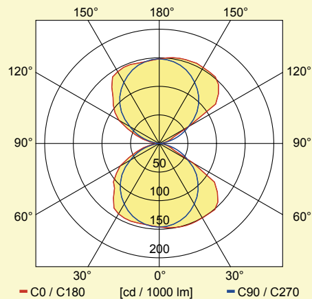
Illustration 98: Applique
