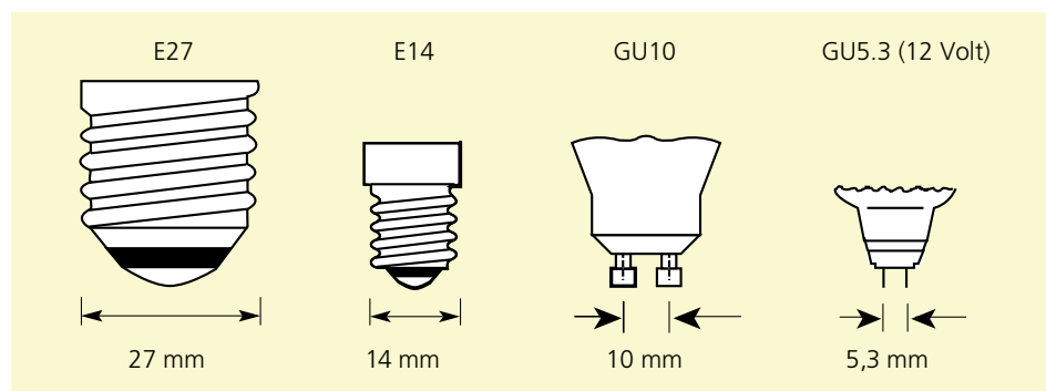
Illustration 155: Types de culot des lampes Retrofit.
